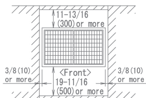
For centralized group layout 《Pattern 1》
