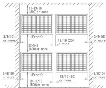
For centralized group layout 《Pattern 1》
