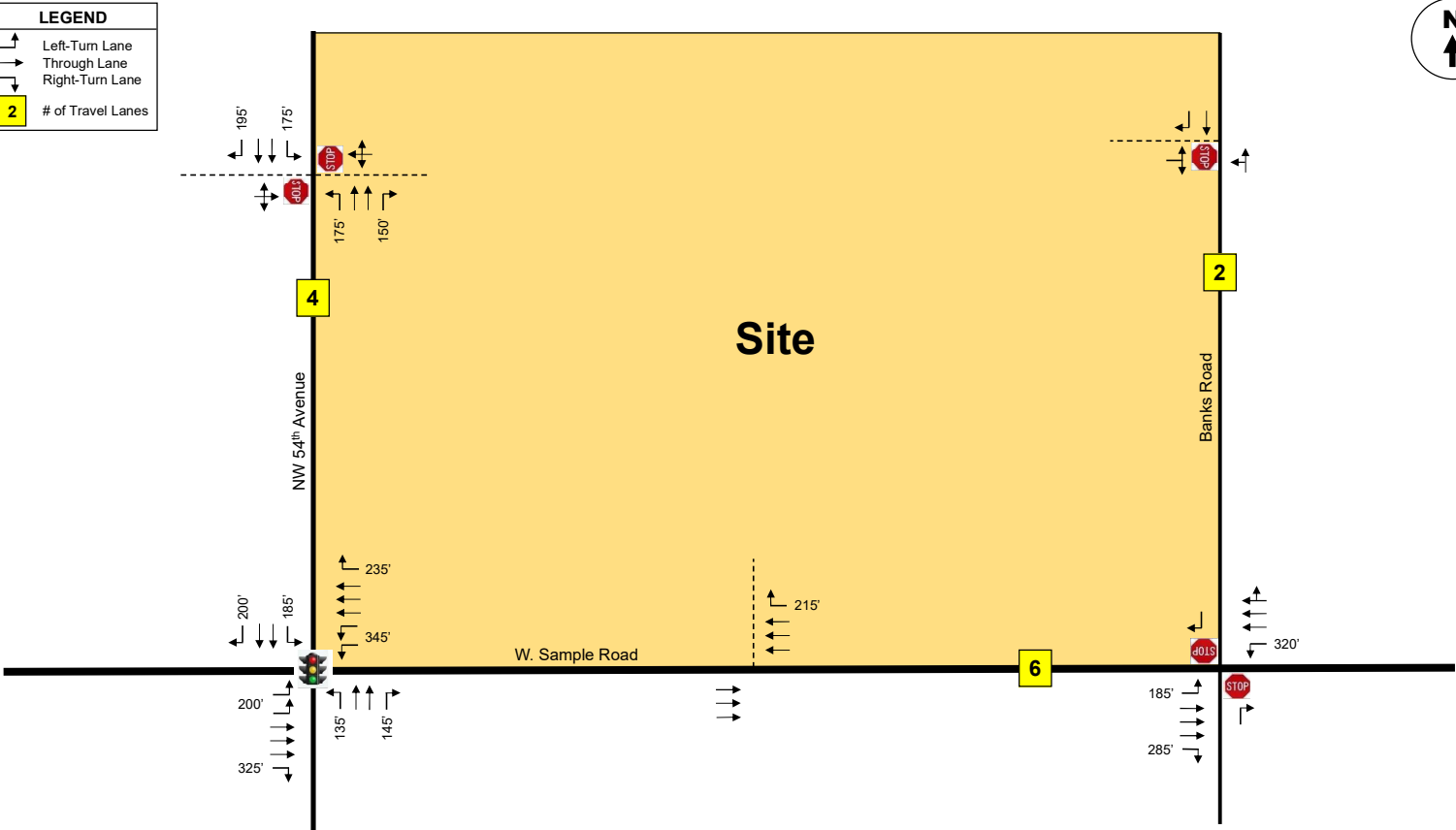
Existing Lane Geometry With Driveway Location & Geometry
