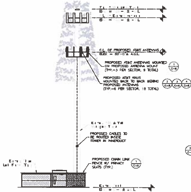
PROPOSED ELEVATION SCALE: 1"=10' FOR 11'x17' 1"=10' FOR 22'x34'
