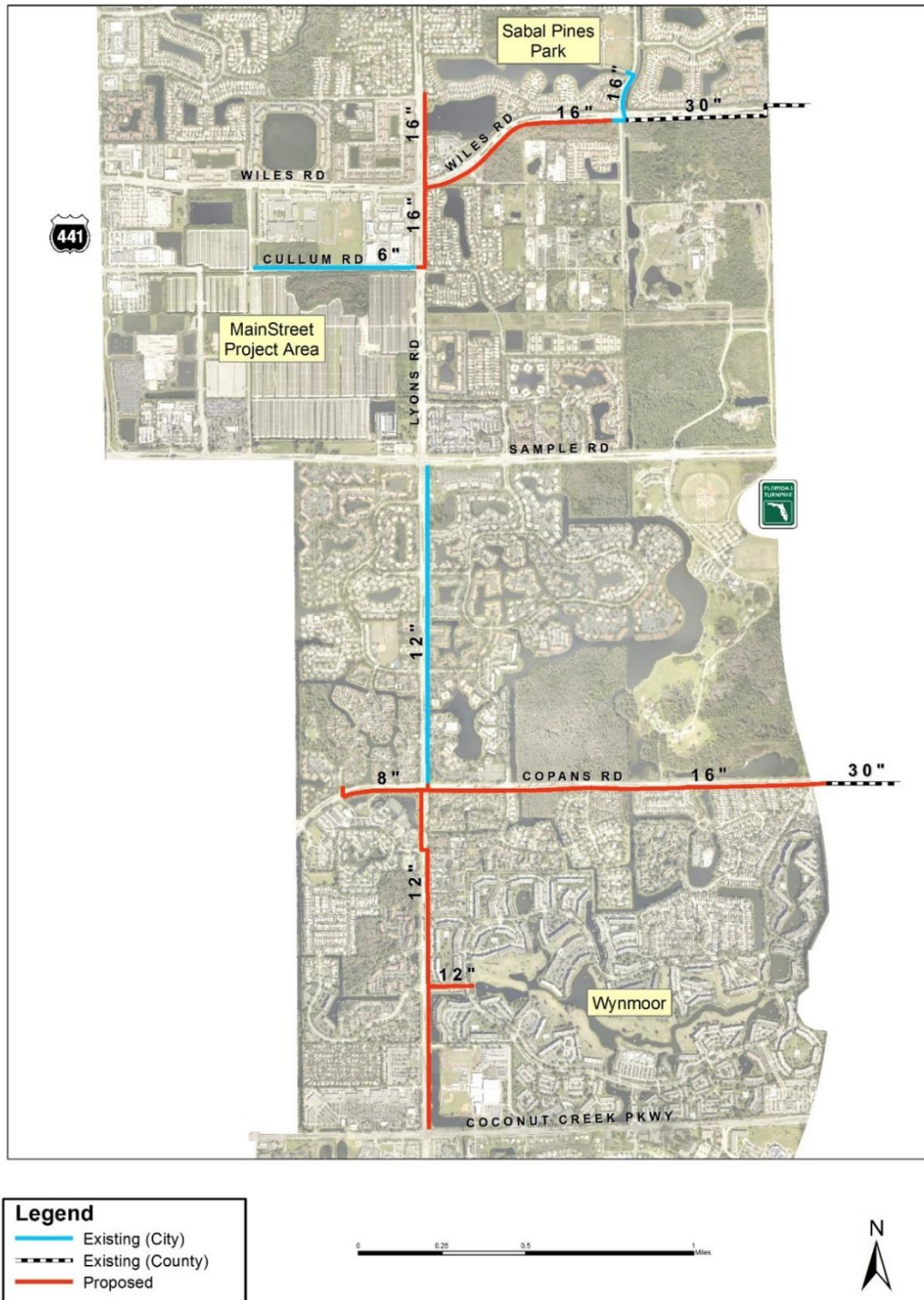
Figure 1. City of Coconut Creek Proposed Reclaimed Watermain Extension
