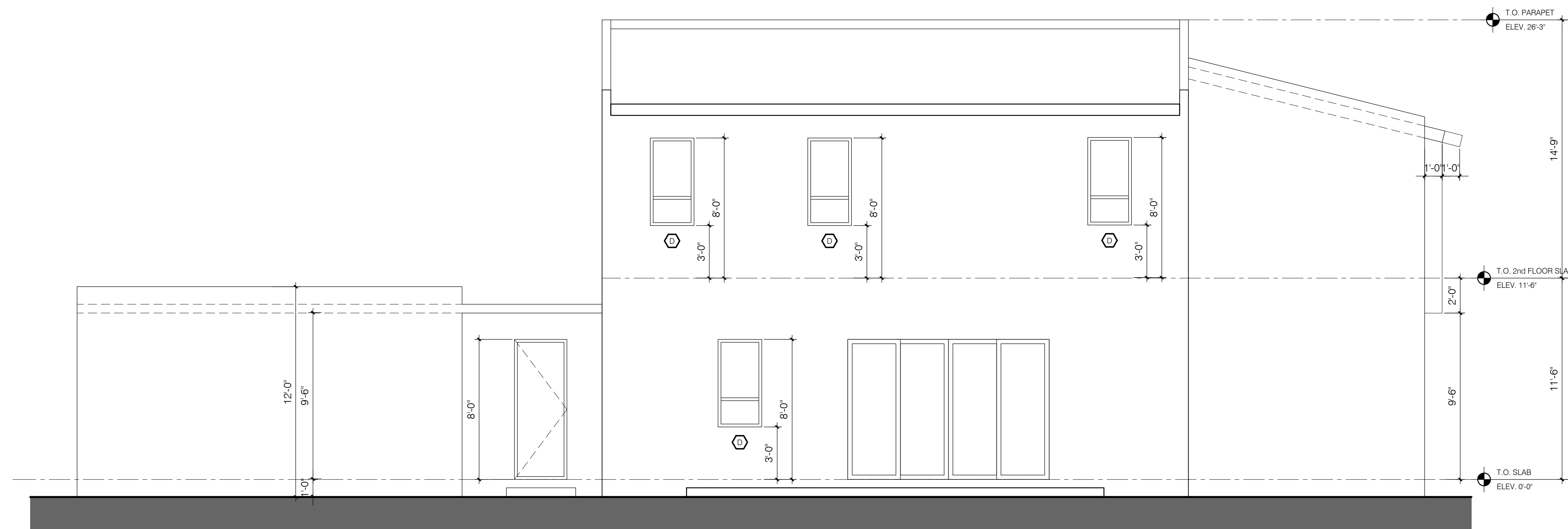
① Rear Elevation 1/4"
