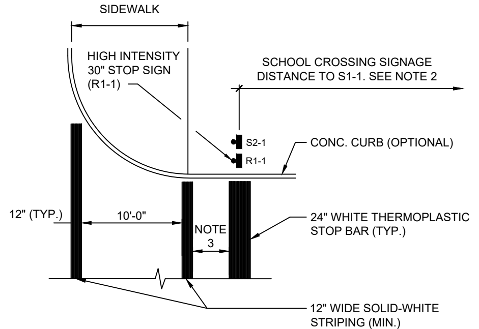
STOP SIGN, STOP BAR, AND SCHOOL CROSSING DETAIL
