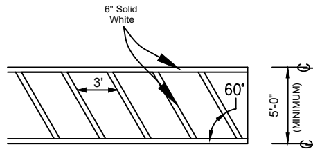
ACCESSIBLE CROSS-WALK DETAIL
