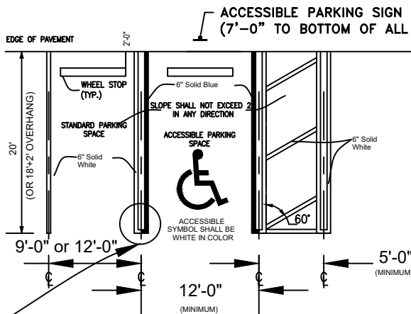
ACCESSIBLE PARKING DETAIL
