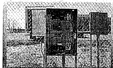
Along a gate using metal tubing to run wiring from one enclosure to another
