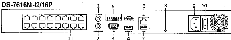
DS-7616NI-I2/16P
