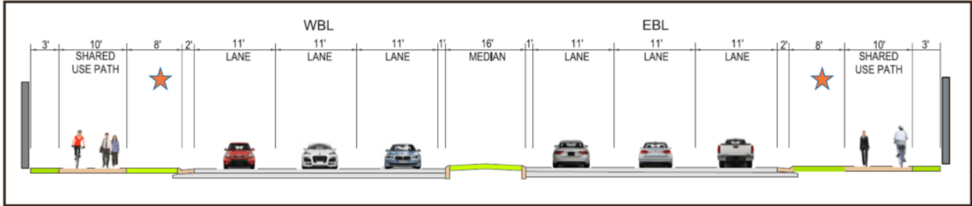
Typical Section
